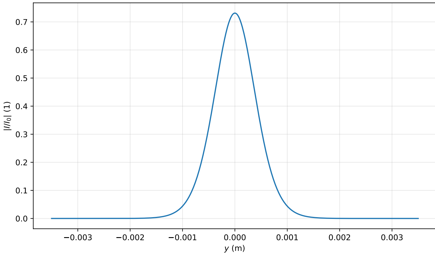
Intensity profile I(x=0, y, z=1.990)/I_0 , P_{in}=0.4P_{cr} , artificial time
